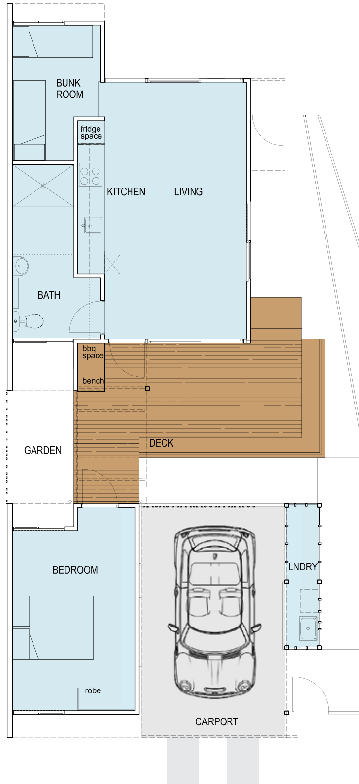
FLOOR PLAN
